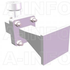
LB-90-10-C-7SPO Standard Gain Horn Antenna 8.2-12.4GHz 10dB Gain 7mm
